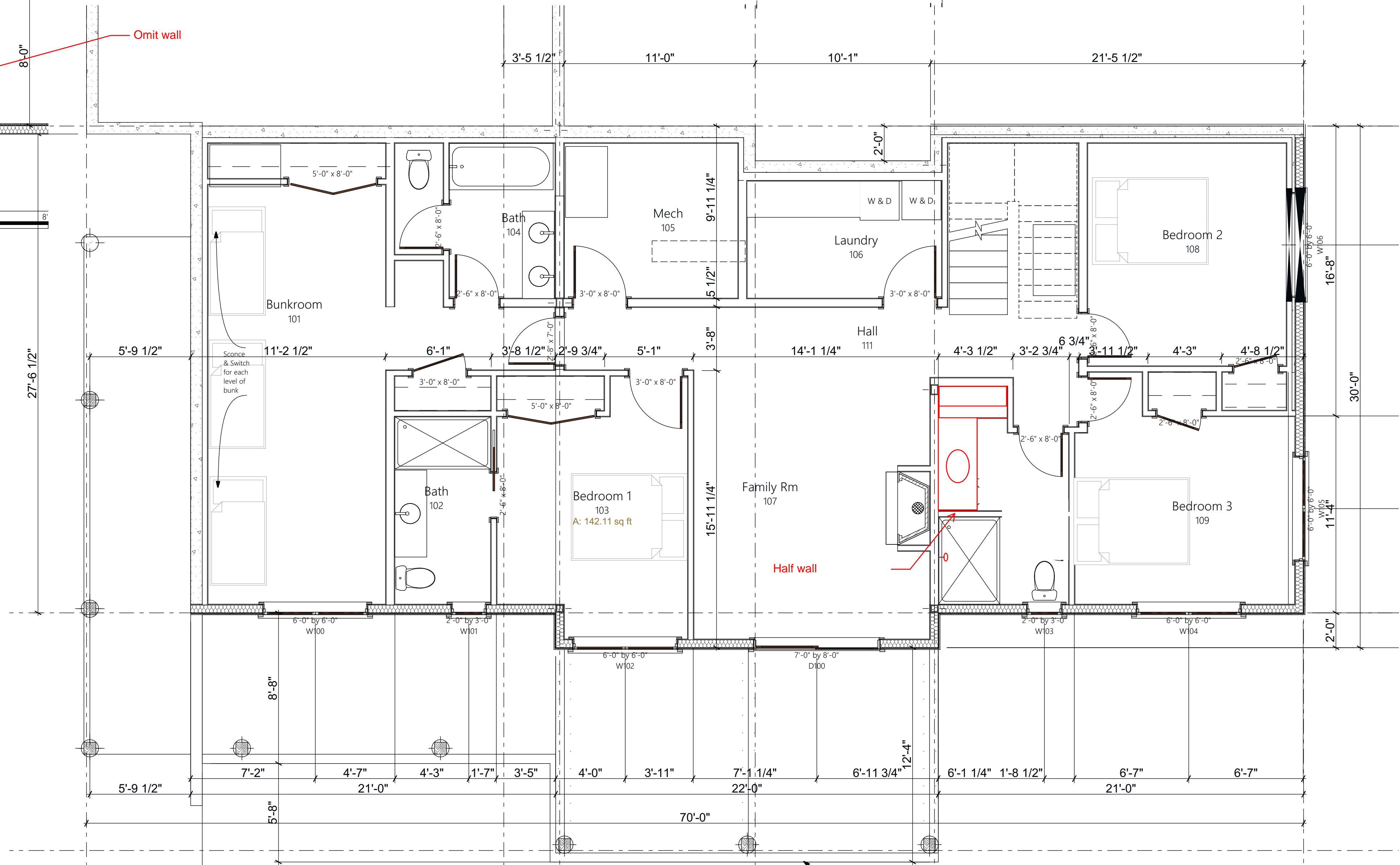
1 Lower Level SCALE: 1/4" = 1'-0"
