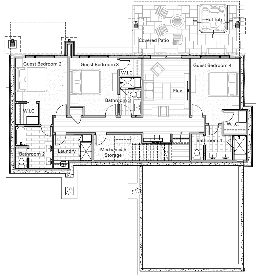
LOWER LEVEL 1,635 SF
